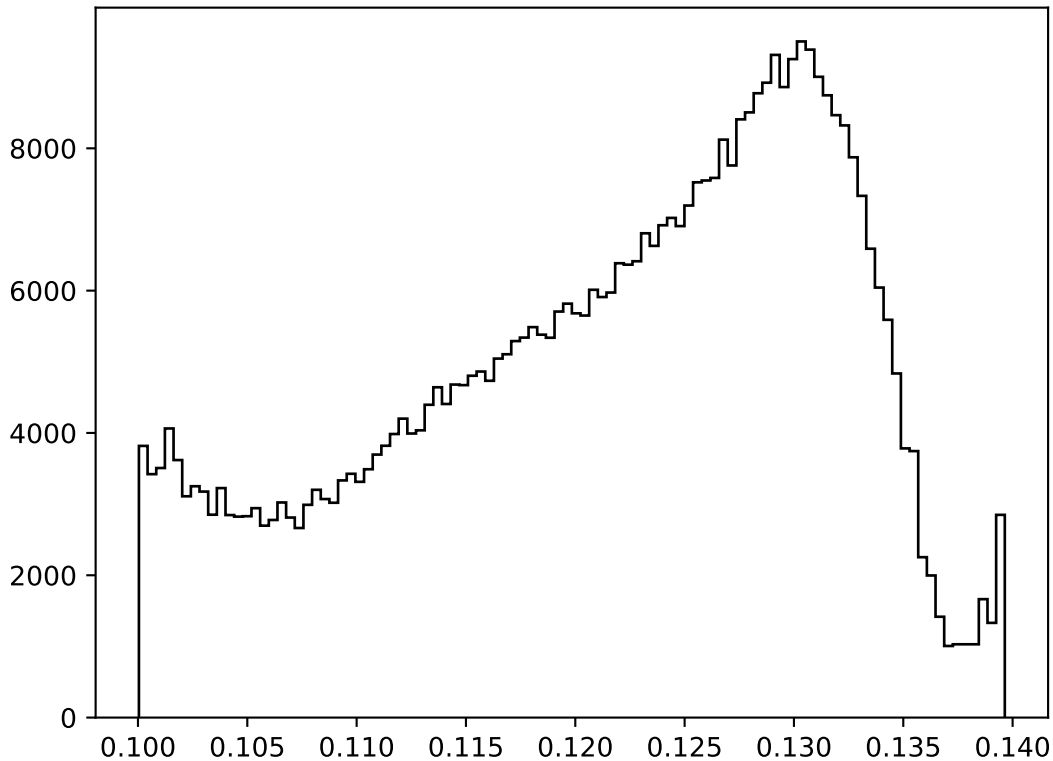
SpaceShower:alphaSvalue=
