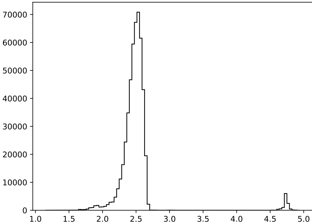
MultipartonInteractions:pT0Ref=
