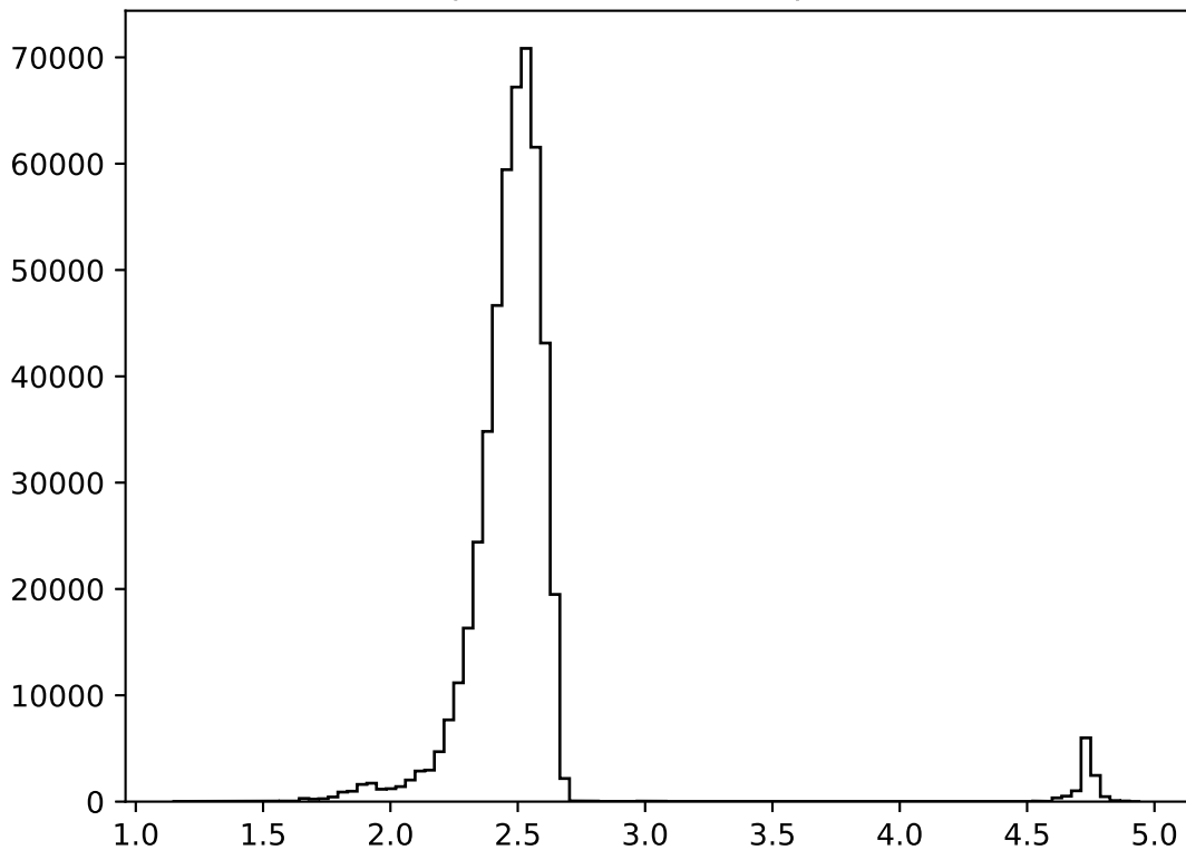
MultipartonInteractions:pT0Ref=
