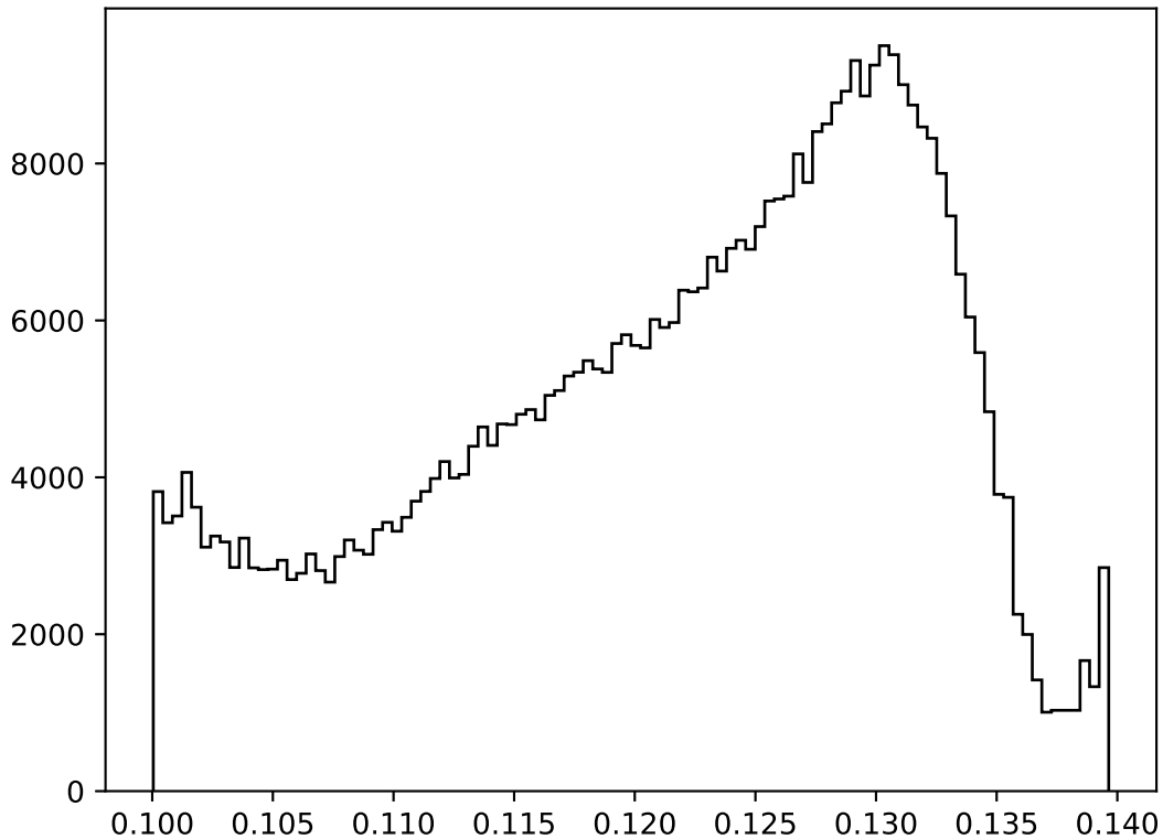
SpaceShower:alphaSvalue=
