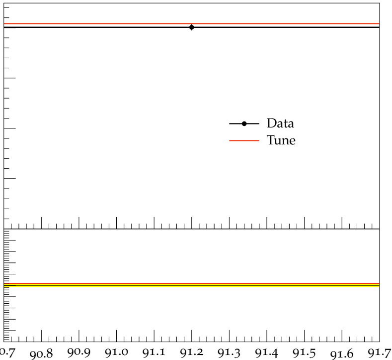
Charged particle multiplicity, ( uds ) events
