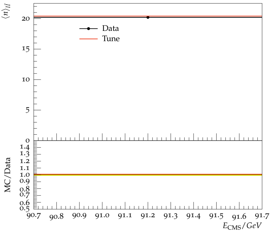
Charged multiplicity in uds events
