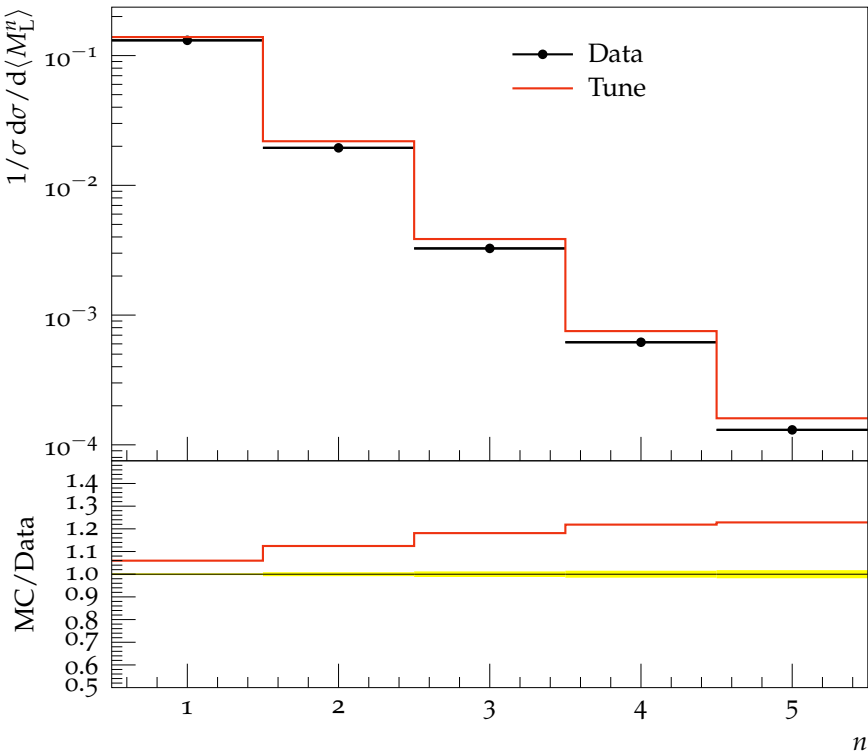
Moments of M_L at 91 GeV
