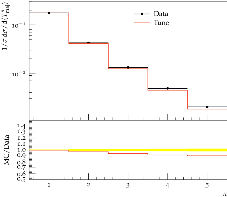
Moments of T_{\text{maj}} at 91 GeV
