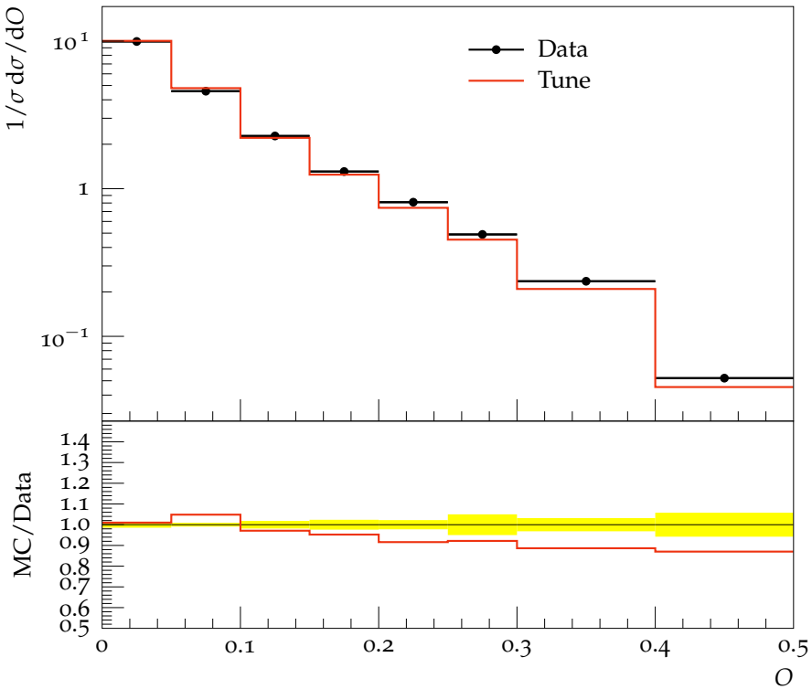
Oblateness, O , at 91 GeV
