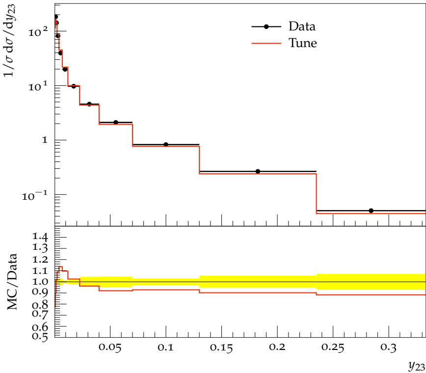
Durham jet 2 \rightarrow 3 transition parameter, y_{23} , at 91 GeV
