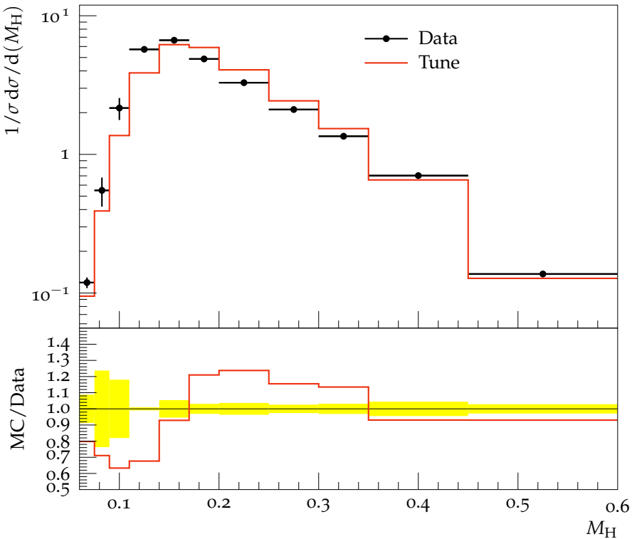
Heavy hemisphere mass, M_H , at 91 GeV
