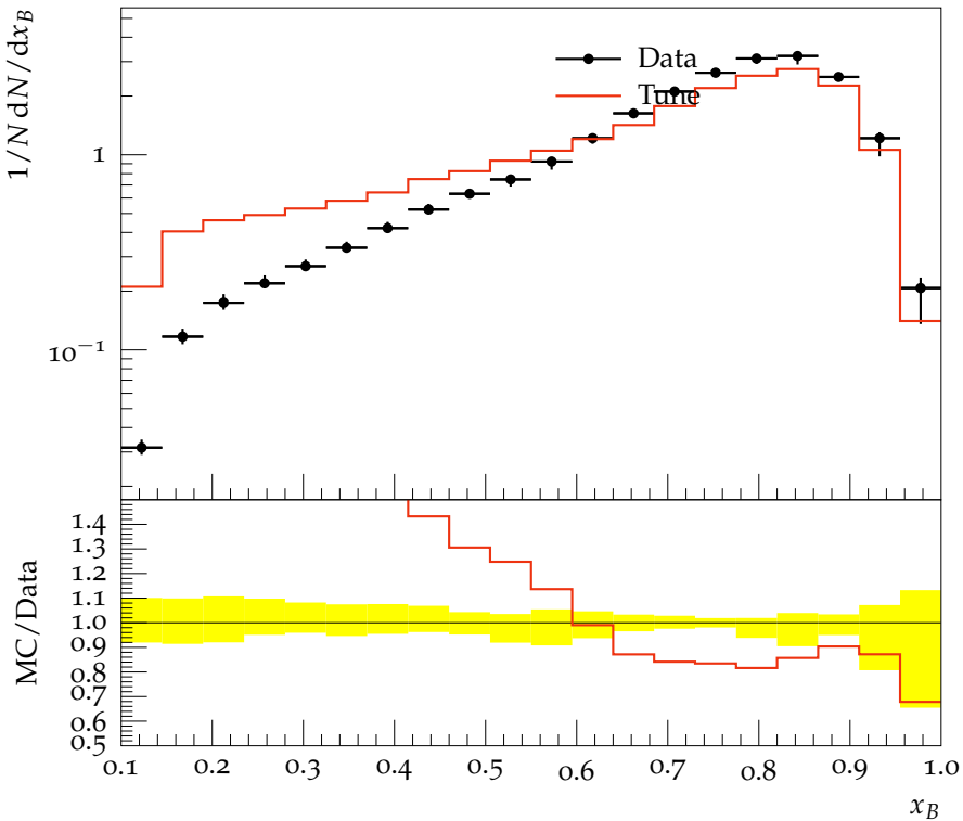
b -quark fragmentation function f(x_B^{weak})
