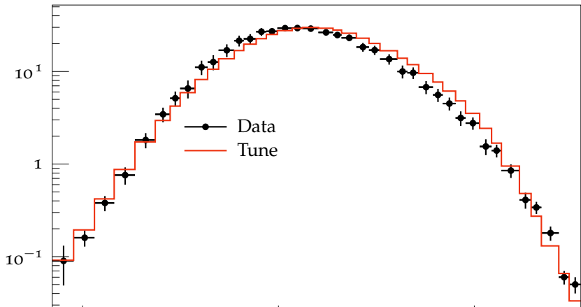
Integrated 5-jet rate with Jade algorithm (91.2 GeV)
