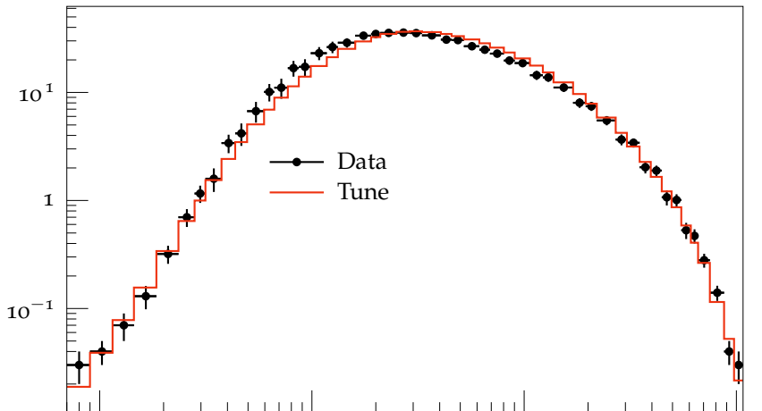
Integrated 4-jet rate with Jade algorithm (91.2 GeV)
