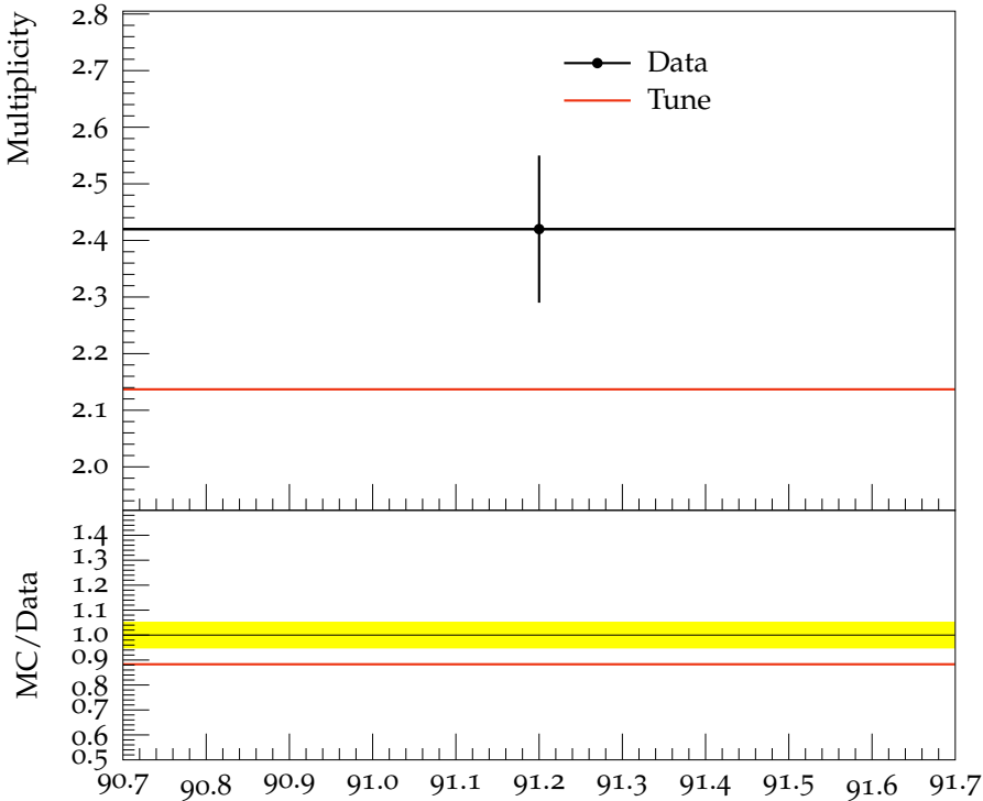
Mean K^+ / K^- multiplicity
