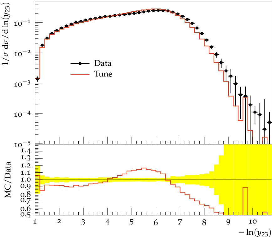
Durham jet resolution 3 \rightarrow 2 ( E_{\text{CMS}} = 91.2 GeV)
