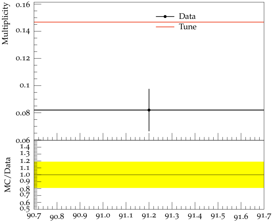
Mean \Sigma multiplicity
