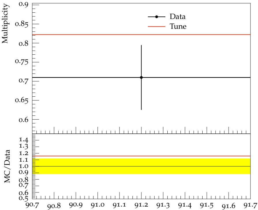
Mean K^{*\pm} multiplicity
