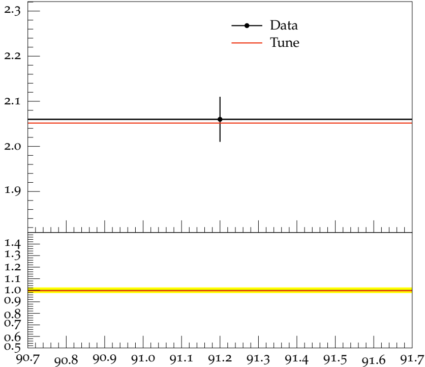
Mean K_S + K_L multiplicity
