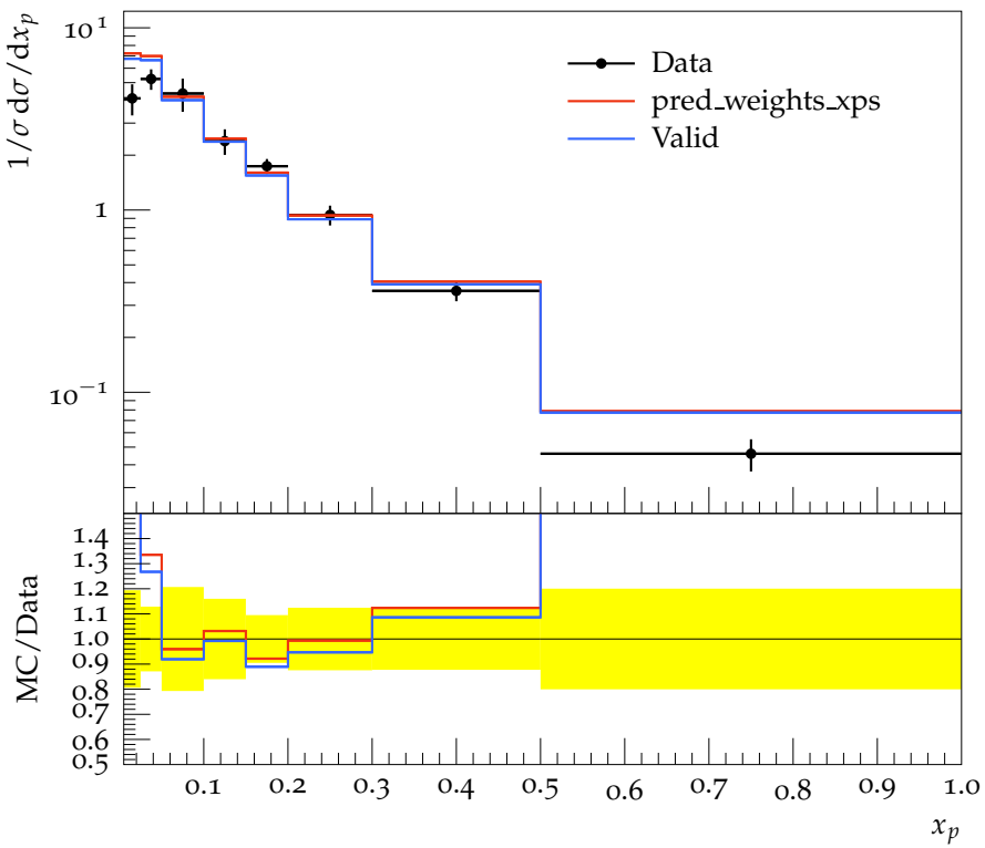
K^{*0}(892) spectrum
