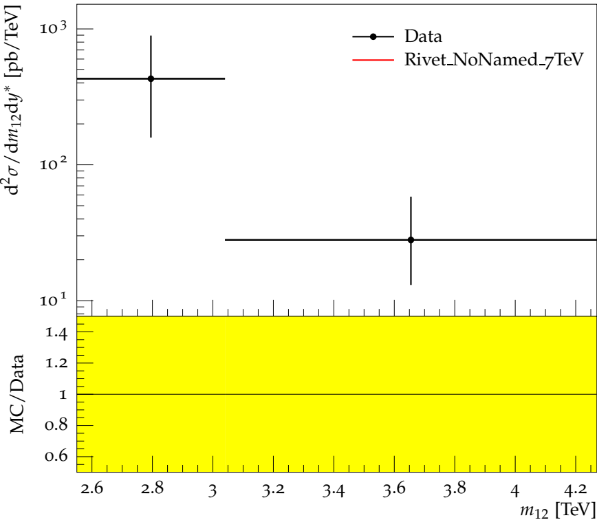
Dijet double-diff. x-section, anti- k_t 0.6 ( 4.0 \leq y^* < 4.4 )
