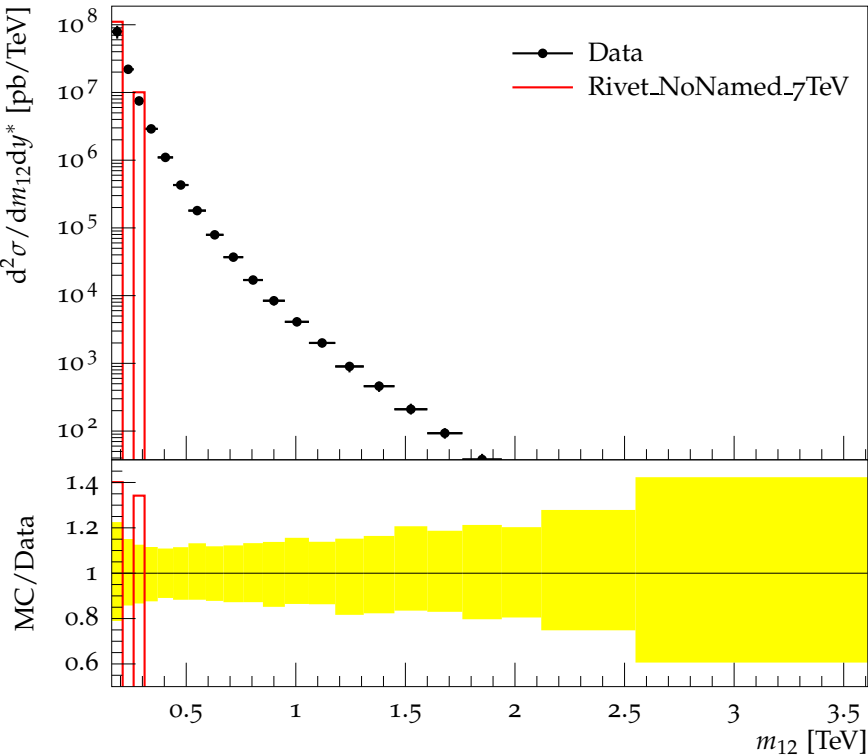
Dijet double-diff. x-section, anti- k_t 0.6 ( 1.0 \leq y^* < 1.5 )
