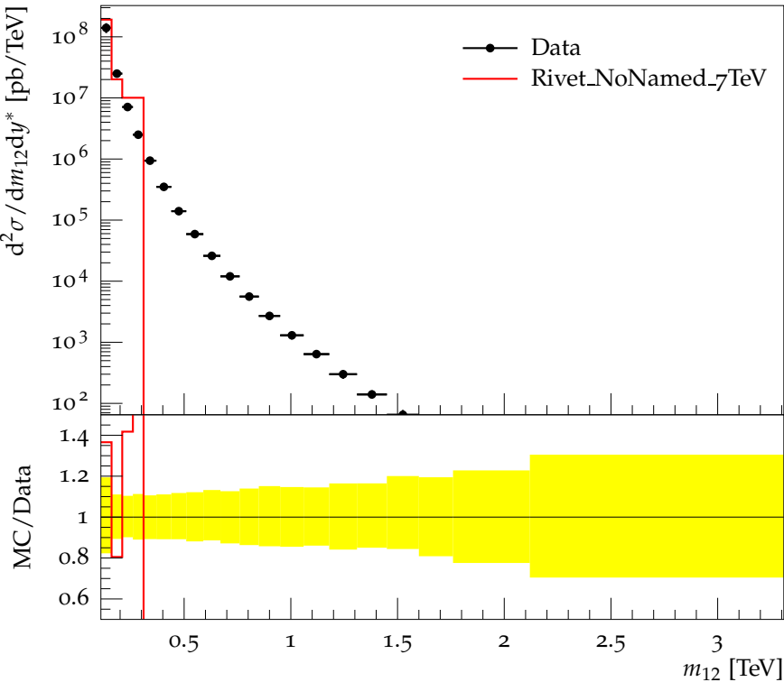
Dijet double-diff. x-section, anti- k_t 0.6 ( 0.5 \leq y^* < 1.0 )
