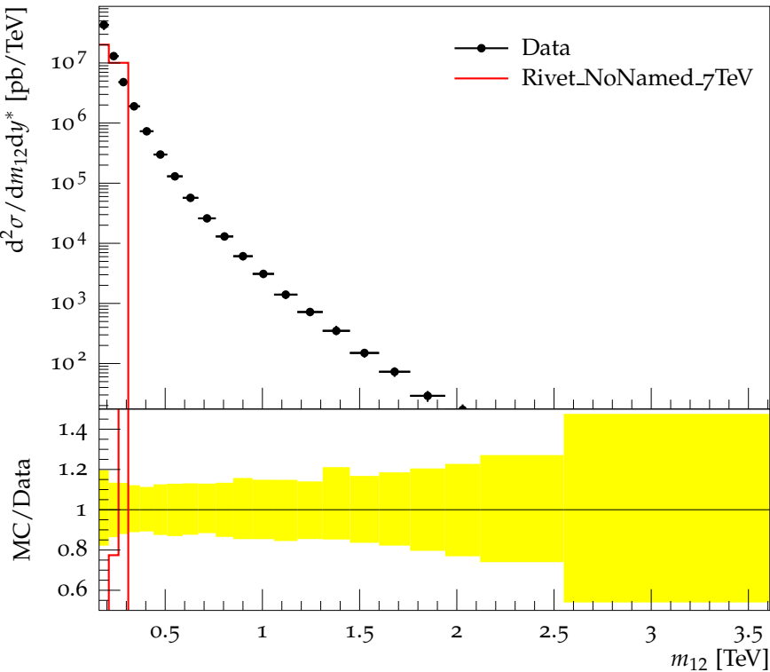
Dijet double-diff. x-section, anti- k_t 0.4 ( 1.0 \leq y^* < 1.5 )
