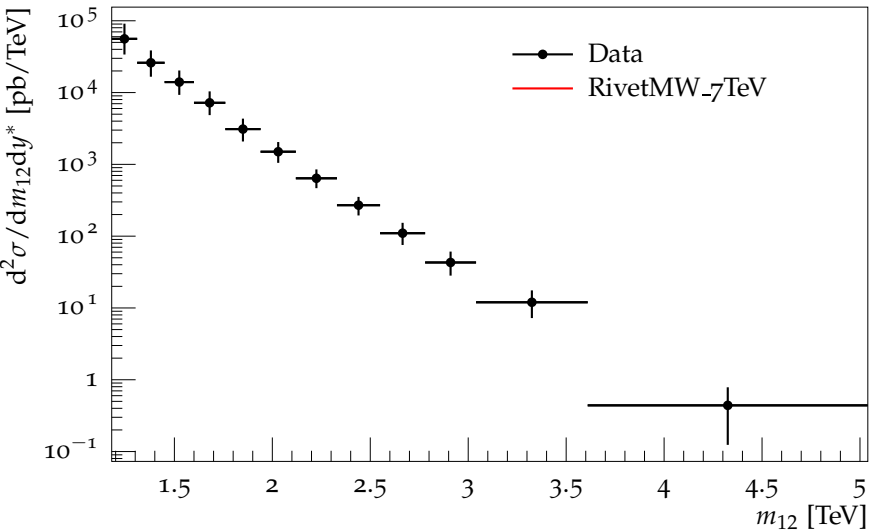
Dijet double-diff. x-section, anti- k_t 0.4 ( 3.0 \leq y^* < 3.5 )
