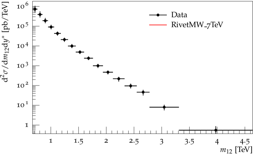
Dijet double-diff. x-section, anti- k_t 0.4 ( 2.5 \leq y^* < 3.0 )
