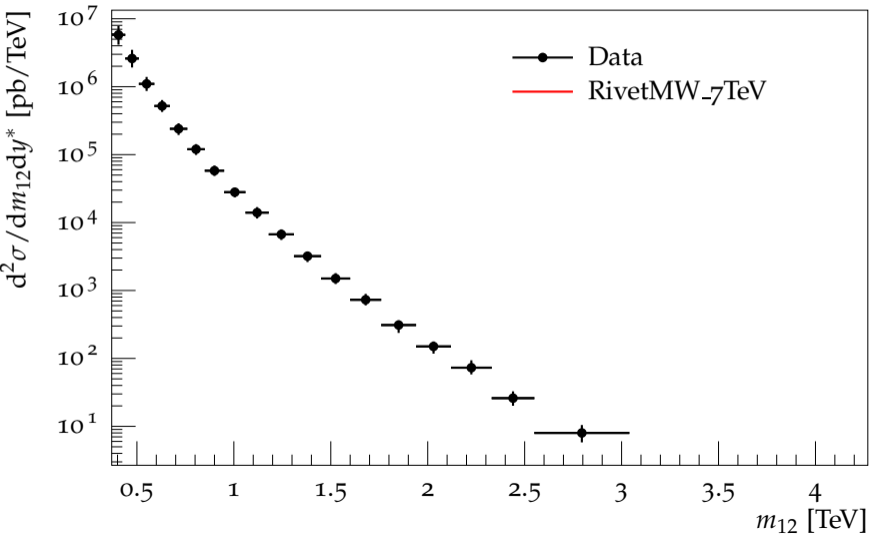
Dijet double-diff. x-section, anti- k_t 0.4 ( 2.0 \leq y^* < 2.5 )
