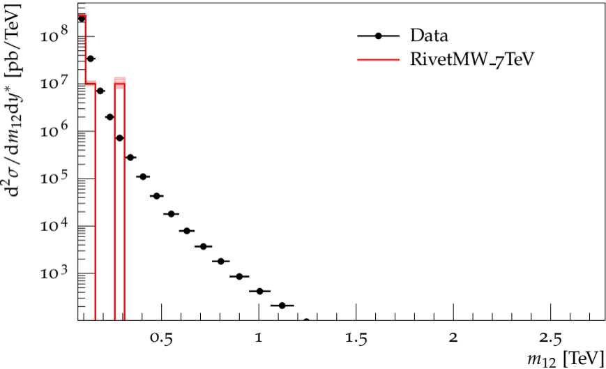
Dijet double-diff. x-section, anti- k_t 0.4 ( y^* < 0.5 )
