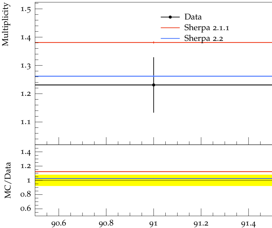
Mean \rho^0(770) multiplicity
