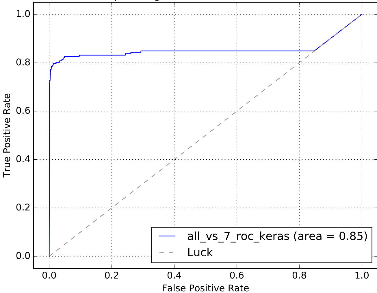
Receiver operating characteristic N0=17135, N1=361
