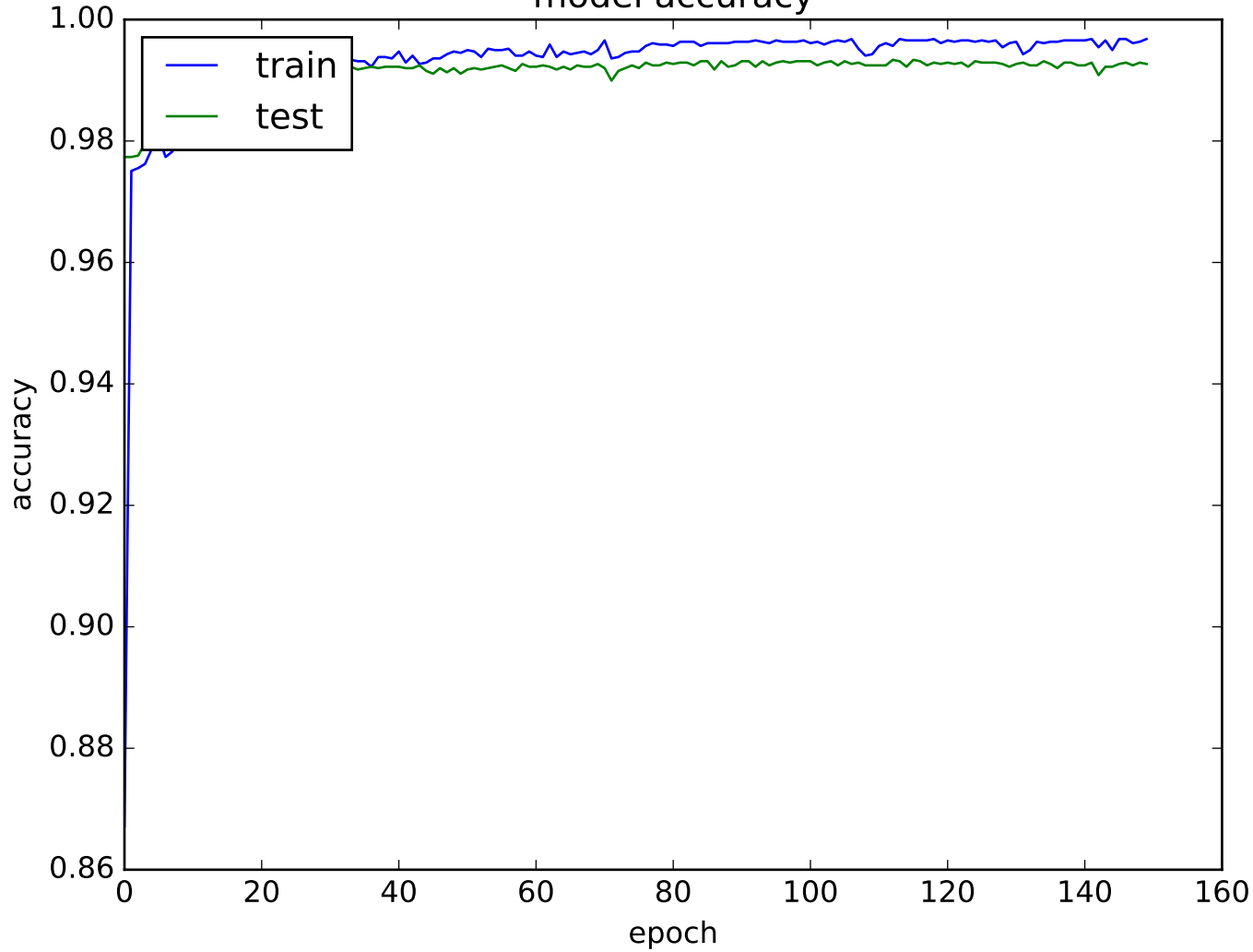
model accuracy
