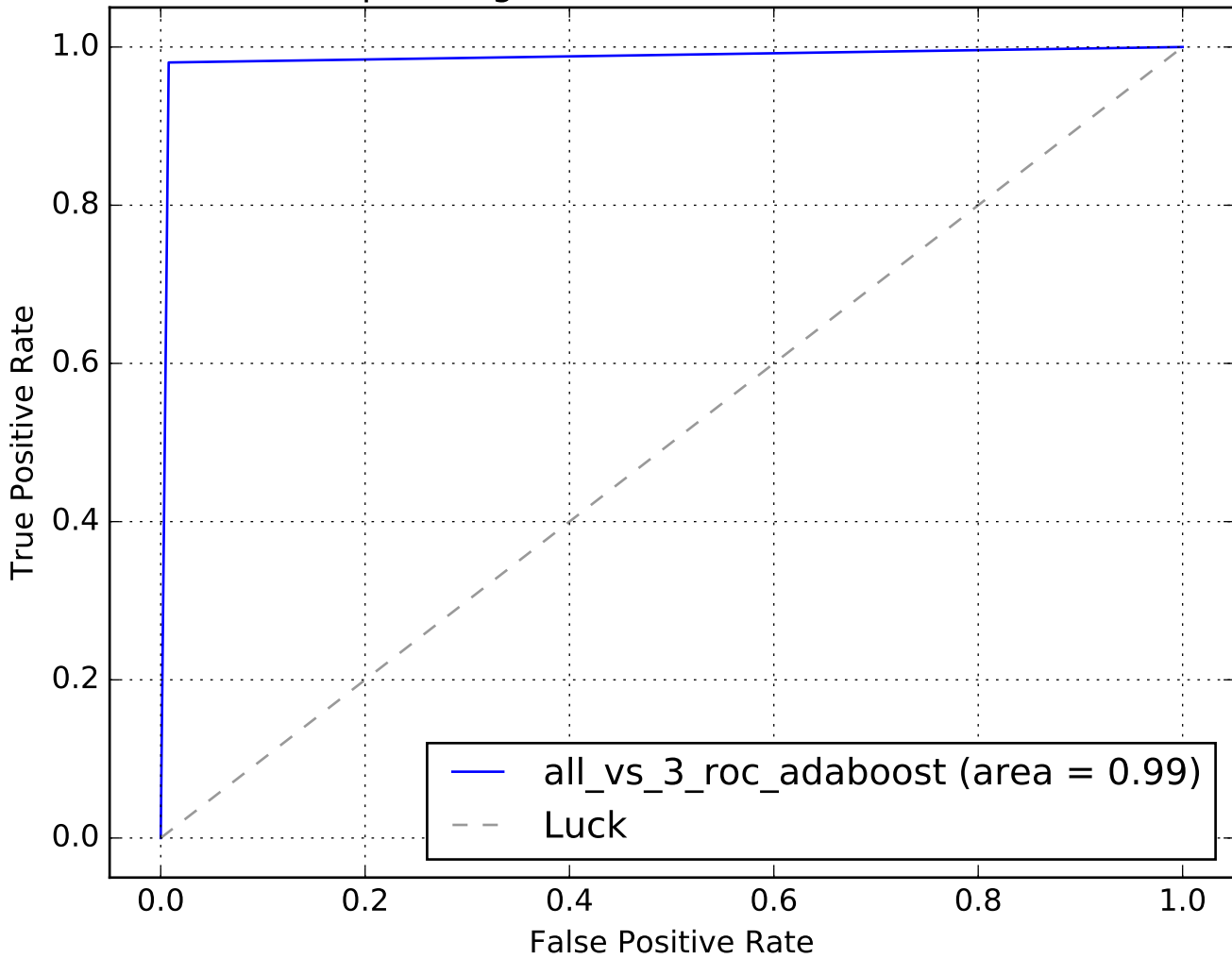
Receiver operating characteristic N0=14152, N1=3344
