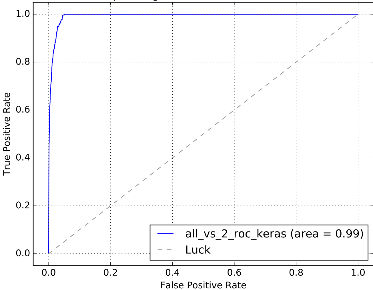
Receiver operating characteristic N0=16810, N1=686
