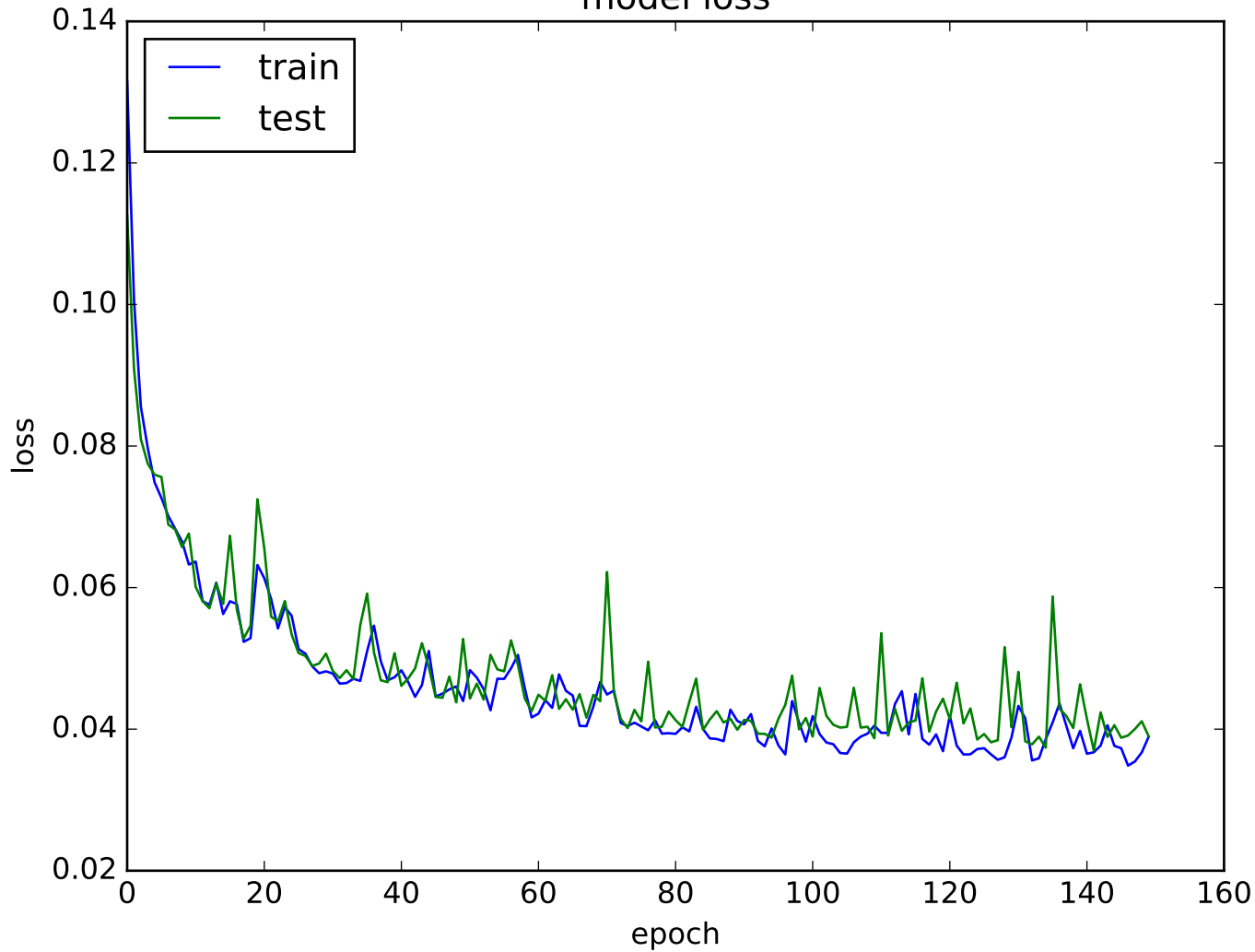
model loss
