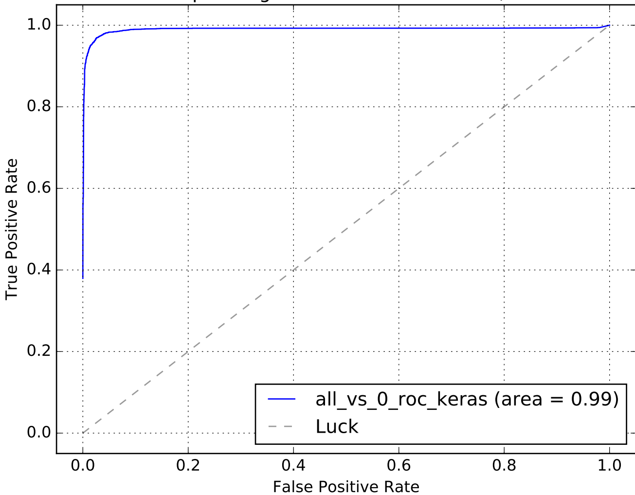
Receiver operating characteristic N0=9890, N1=7606
