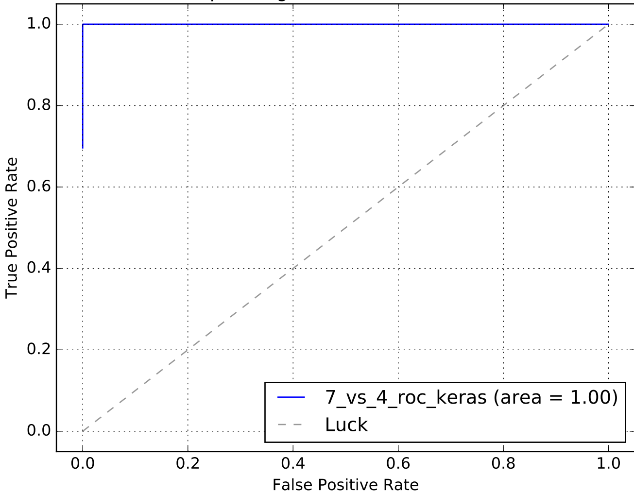
Receiver operating characteristic N0=64, N1=361
