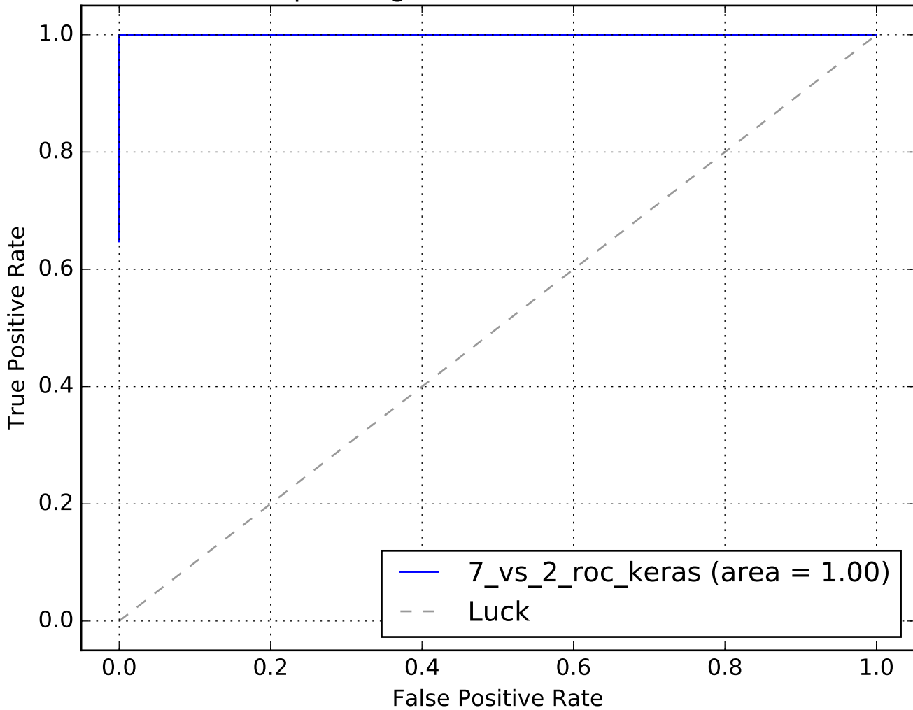
Receiver operating characteristic N0=686, N1=361
