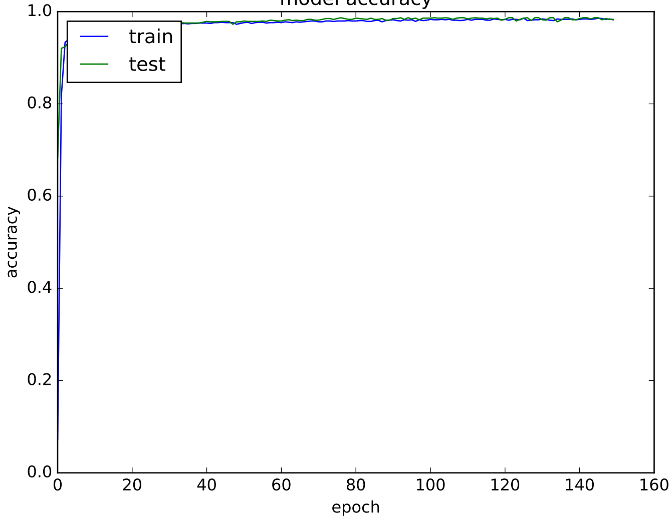
model accuracy
