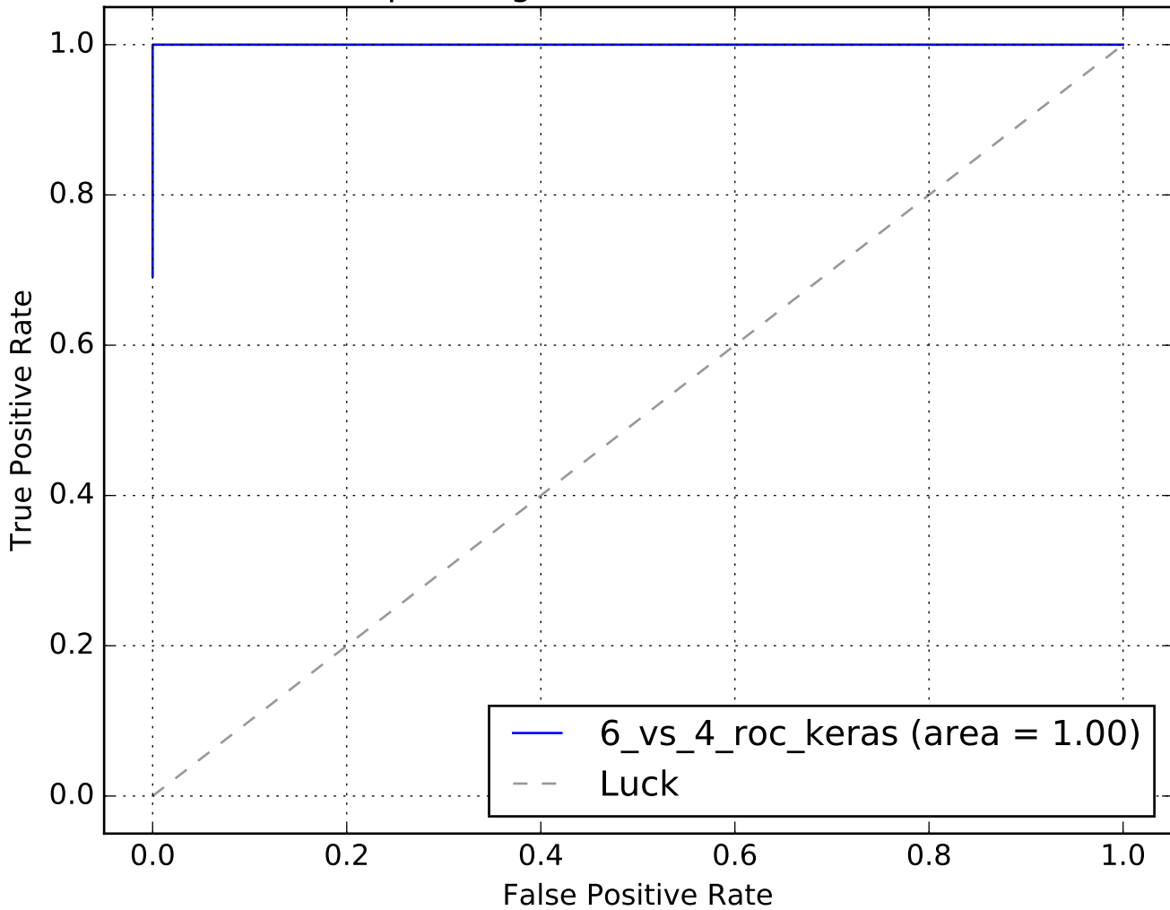
Receiver operating characteristic N0=64, N1=665
