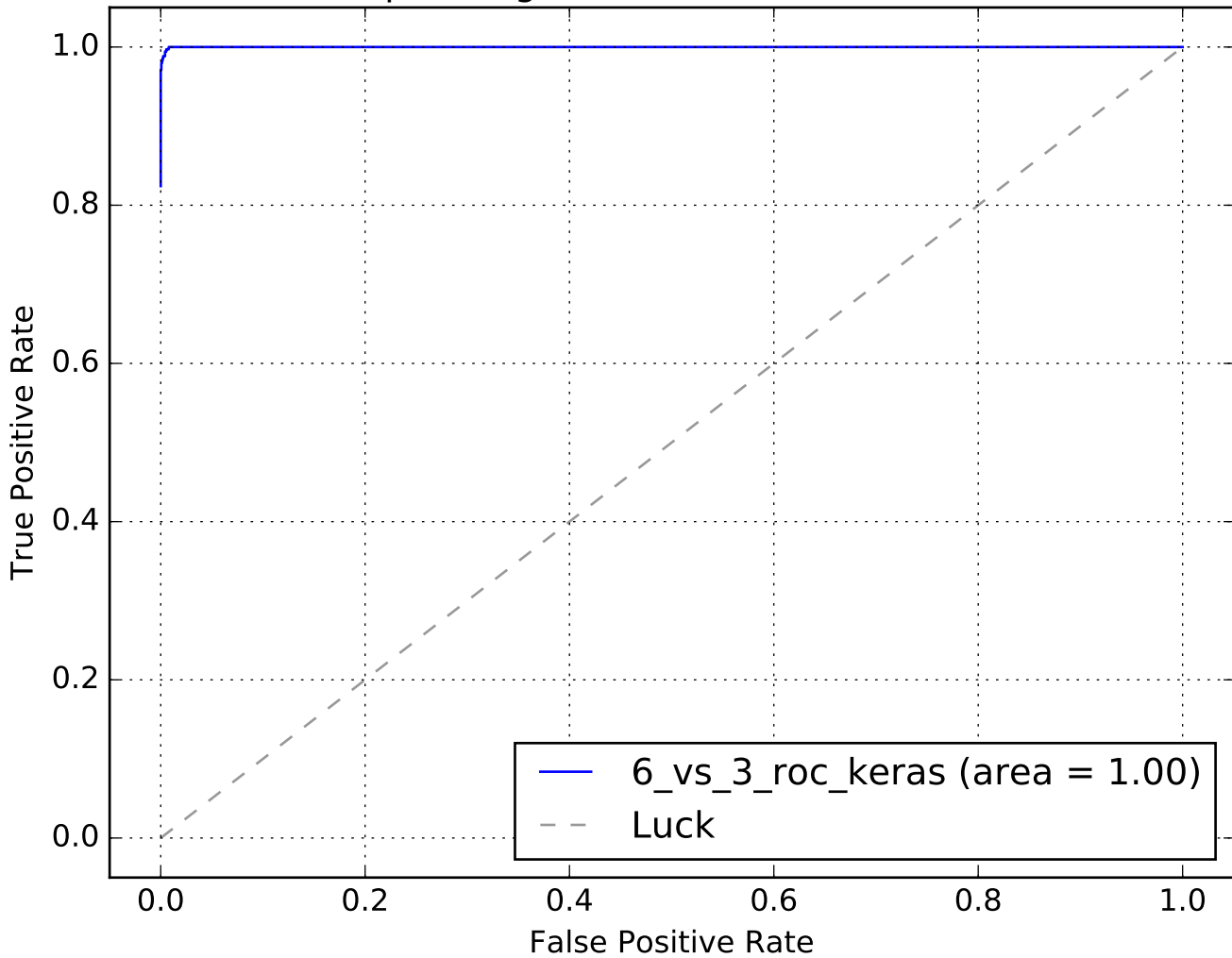
Receiver operating characteristic N0=3344, N1=665
