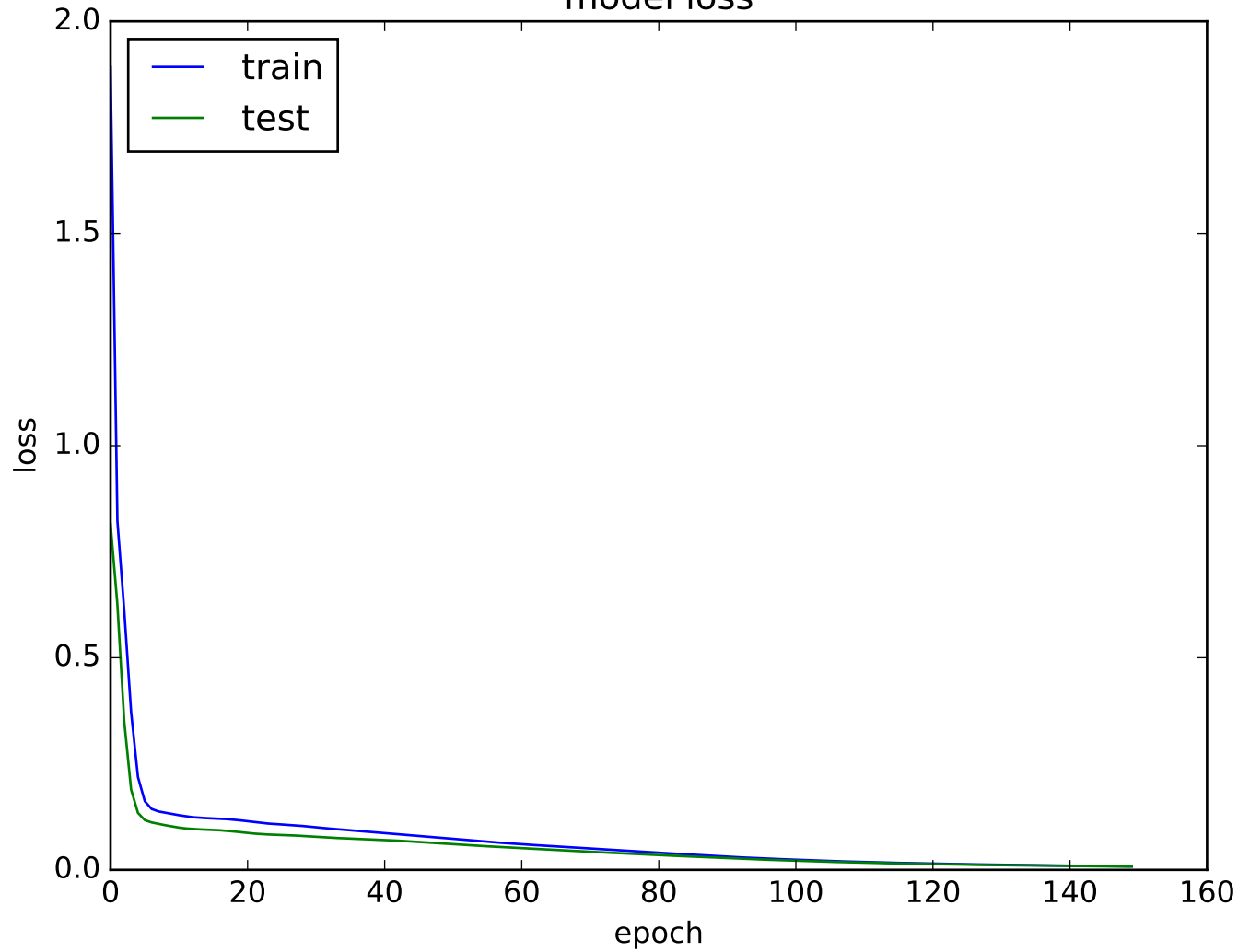
model loss
