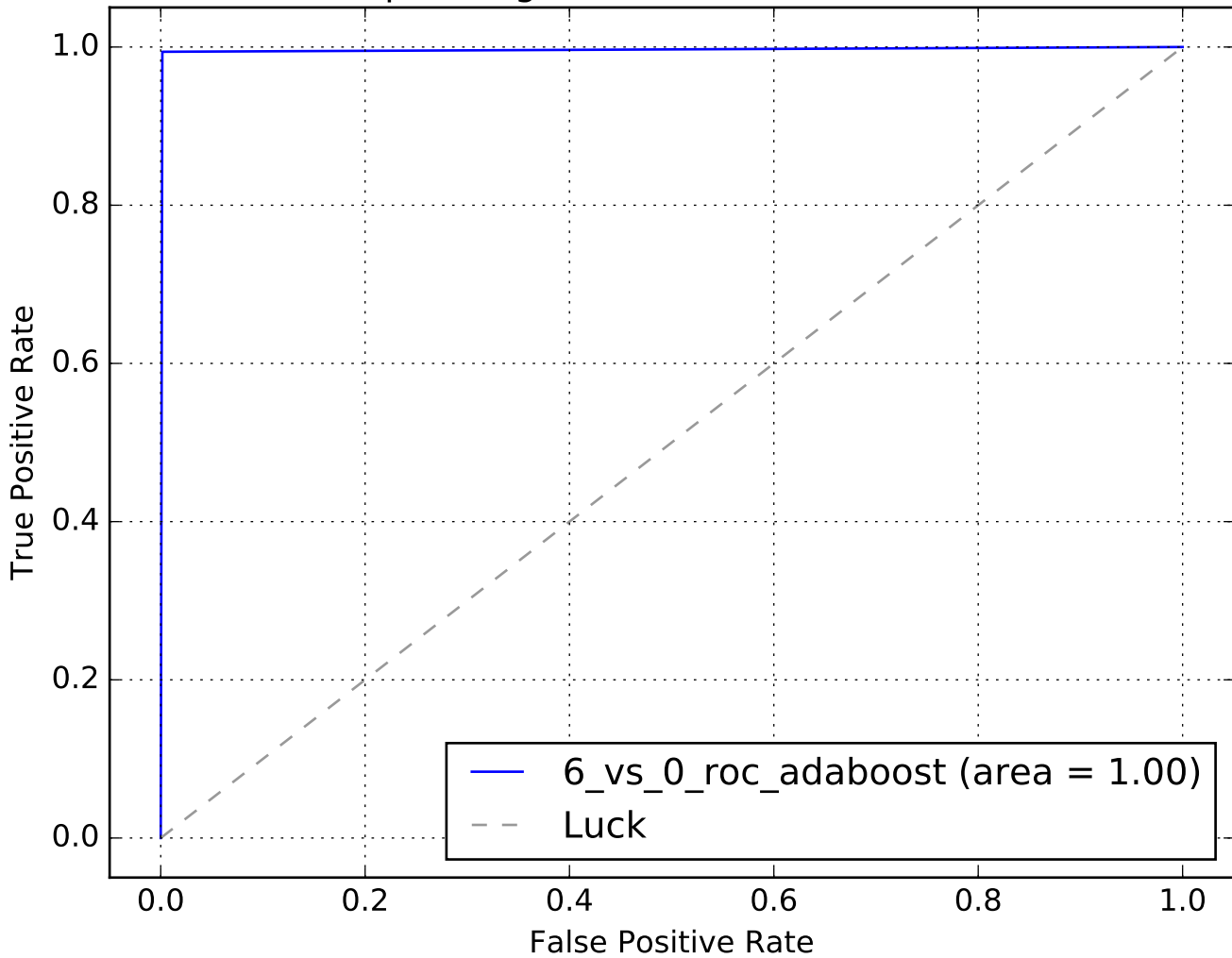
Receiver operating characteristic N0=7606, N1=665
