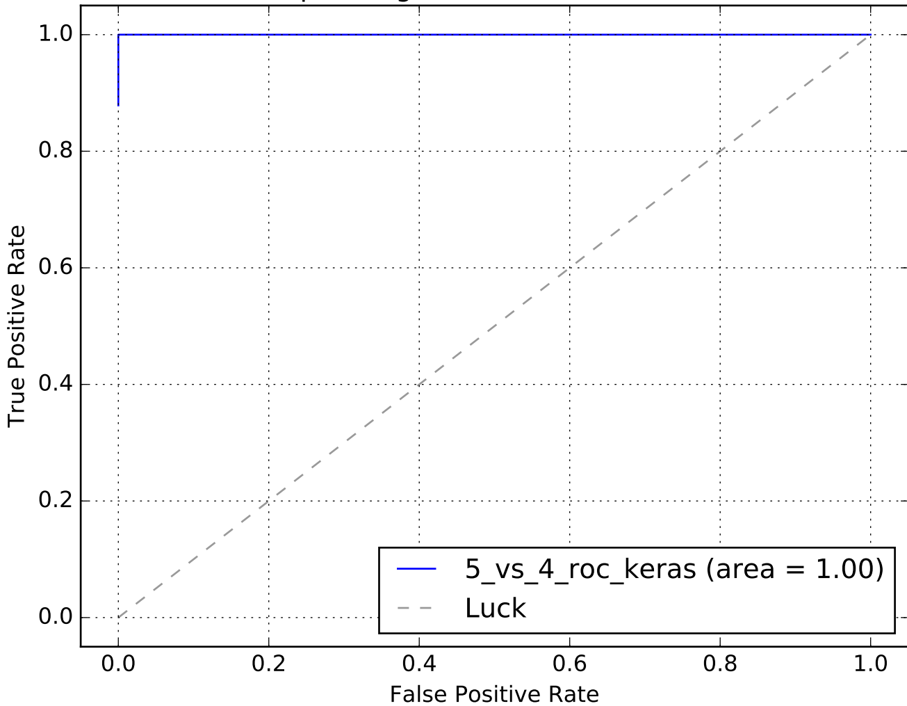
Receiver operating characteristic N0=64, N1=611
