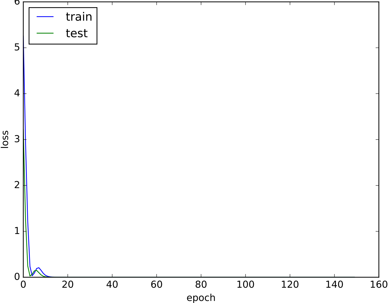
model loss
