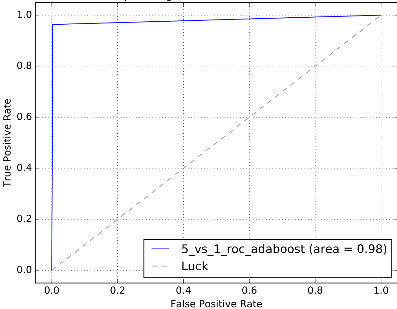
Receiver operating characteristic N0=4159, N1=611
