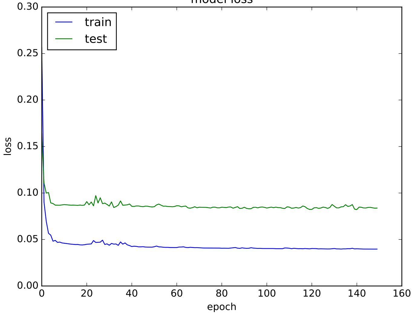
model loss
