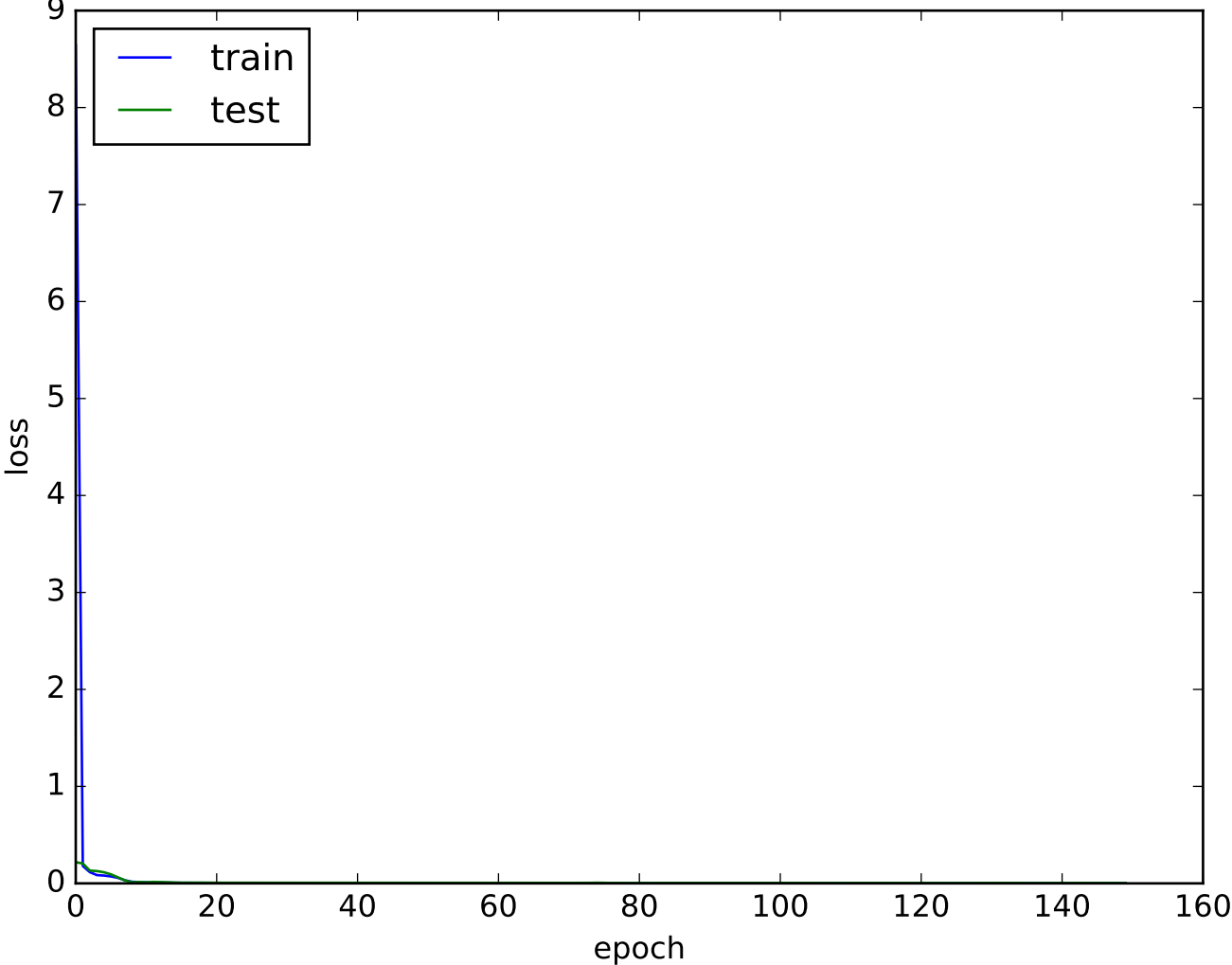
model loss
