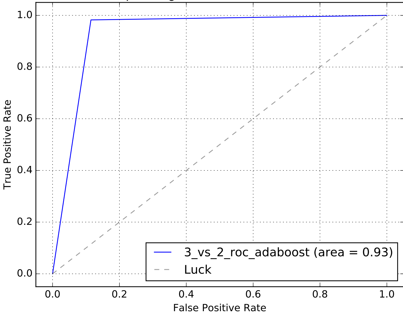
Receiver operating characteristic N0=686, N1=3344
