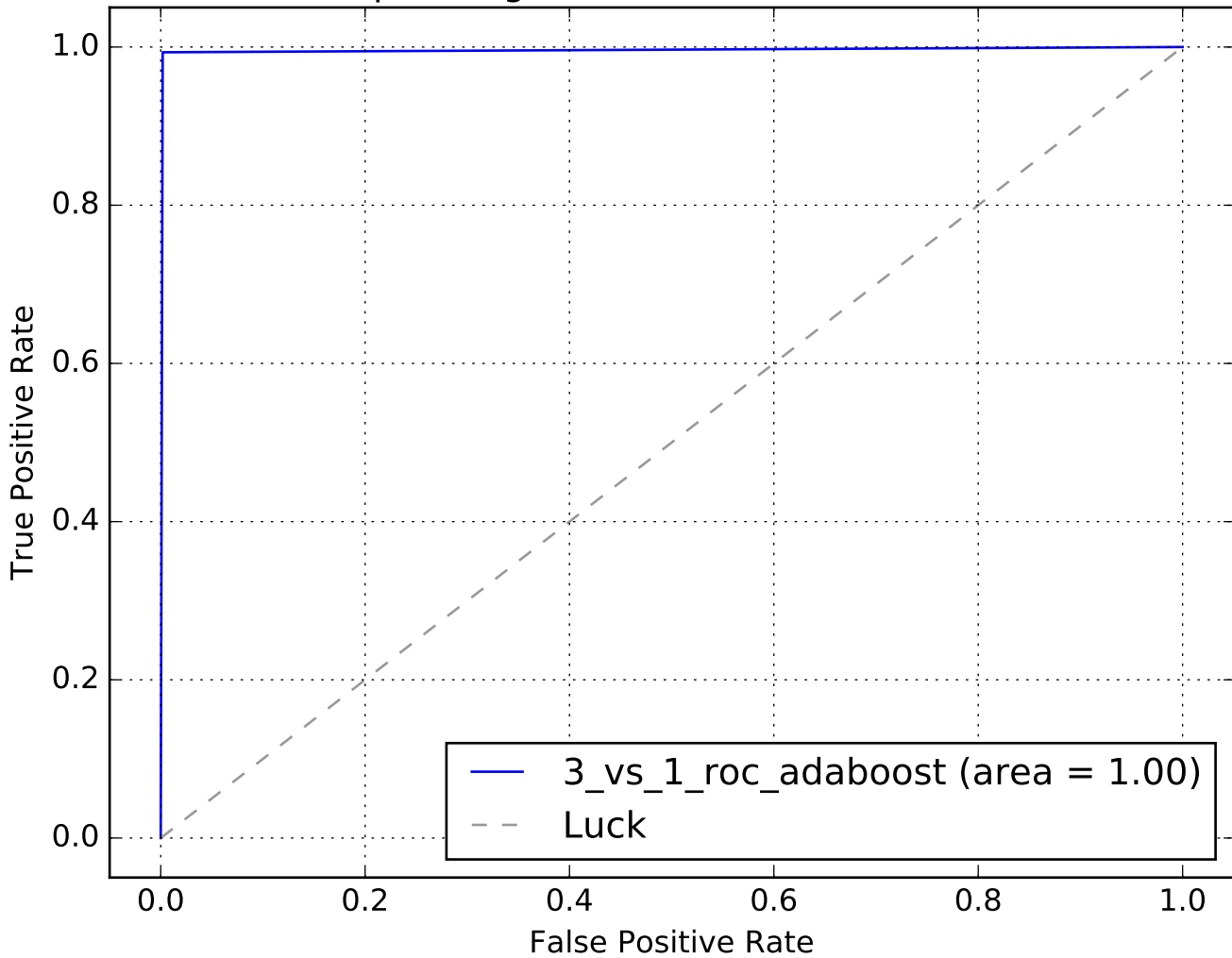
Receiver operating characteristic N0=4159, N1=3344
