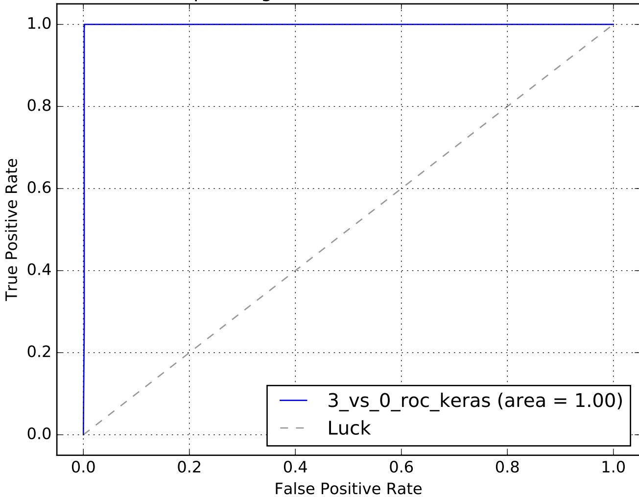
Receiver operating characteristic N0=7606, N1=3344
