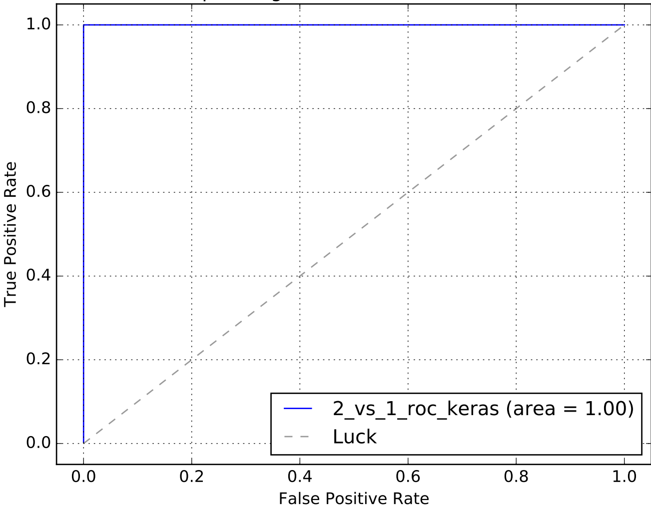
Receiver operating characteristic N0=4159, N1=686
